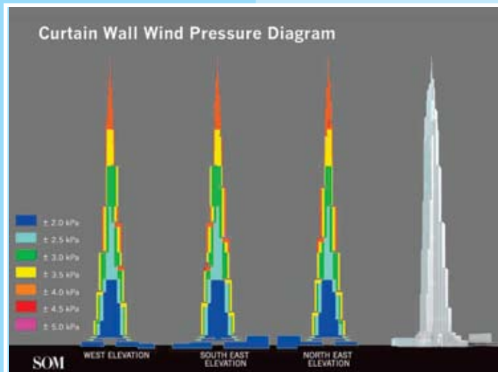
Figure 5: Cladding Pressure Wind Load Diagrams
