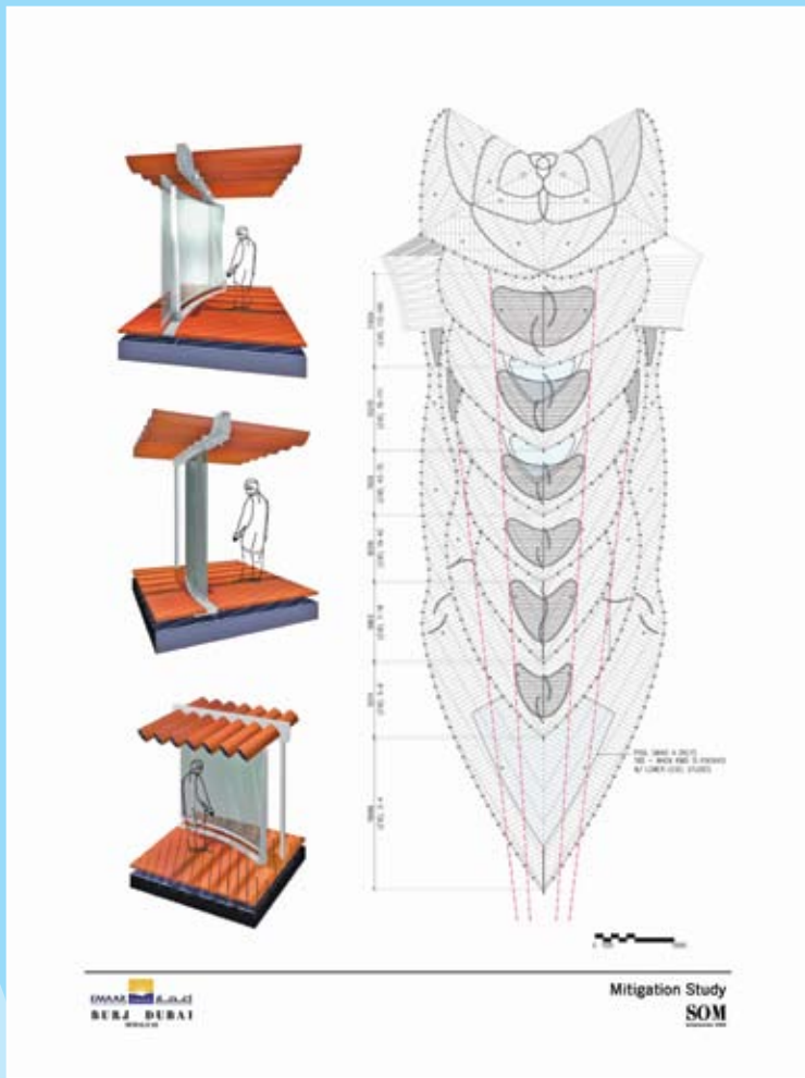
Figure 9a: Divider Screen Design and Terrace Layouts
