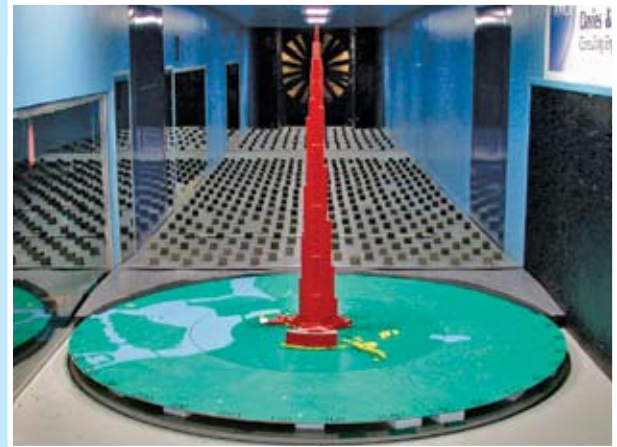
Figure 7a: Pedestrian Level Wind Tunnel Study (without surrounding future structures)
