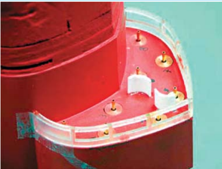
Figure 8c: Divider Screens with Modified Parapet
