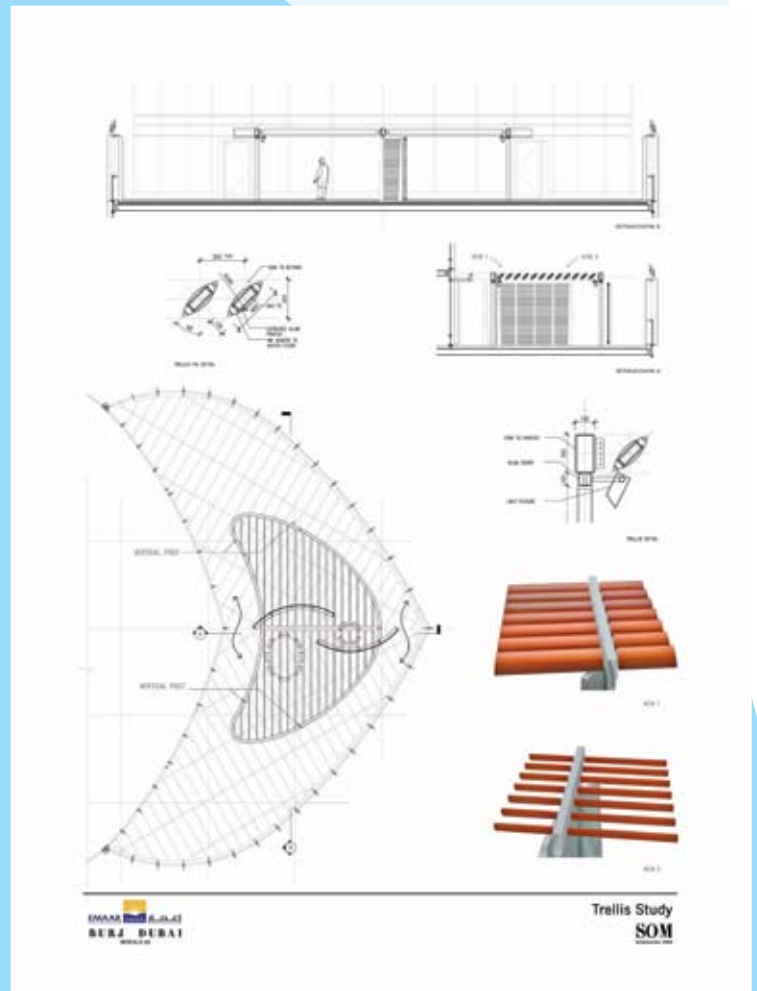
Figure 9b: Plan and Section through Terrace and Trellis Details
