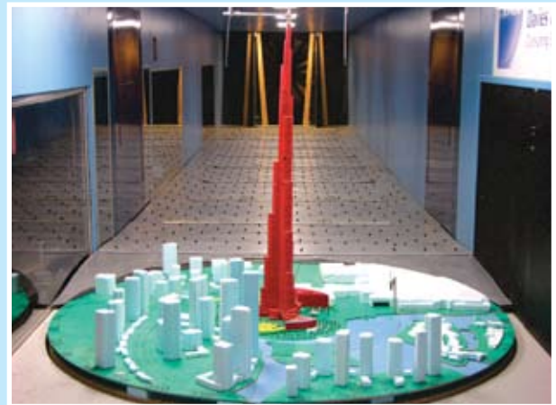
Figure 7b: Pedestrian Level Wind Tunnel Study (with surrounding future structures)
