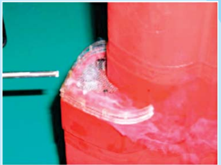
Figure 8d: Smoke Visualization Testing: Divider Screens and Trellis with Modified Parapet
